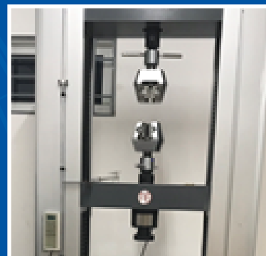
Testing equipment of metal material pulling load 100kN Model: WDW-100E (Origin: Jinan - China)
